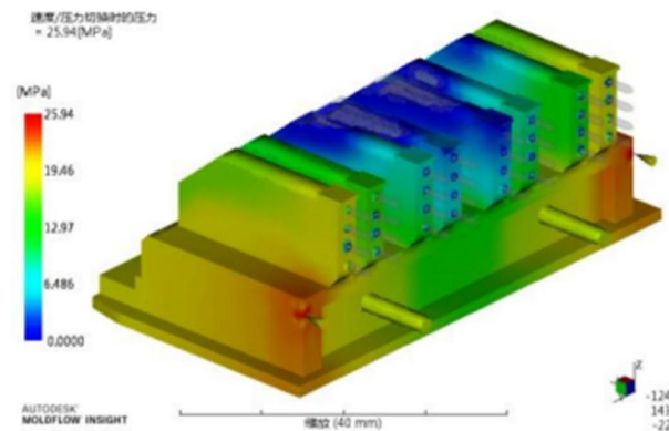
Pressure at V/P switchover(V/P转换及其压力分布)
