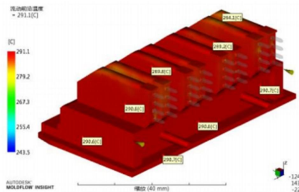
Front Temp before flowing(熔体流动前沿温度)
