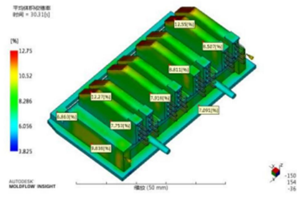
Volume shrinkage at ejection(顶出时体积收缩)
